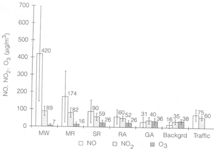
Fig. 1. NO, NO 2 and O 3 concentrations in different land use types in Essen, Germany (Air hygienic profile measurements, 12 trips, 1995) (Kuttler, Straßburger 1997) MW – Motorway, MR – Main road, SR – Side road, RA – Residential area, GA – Green area, Background and traffic stations of the North Rhine-Westphalia State Environment Agency
