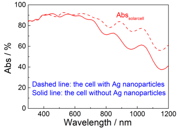
Fig.4 Absorption of the complete cells ( Abs_{solarcell} ) with and without Ag incorporation
