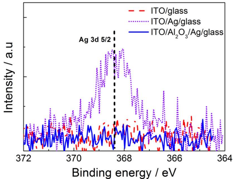
Fig.2 Investigation of Ag diffusion after the CIGSe deposition
