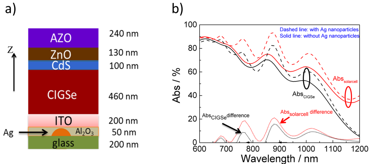
Fig.5 a) Cross section of the unit cell in the finite element method (FEM) simulation; b) simulation of Abs_{CIGSe} and Abs_{solarcell} with and without Ag nanoparticles at the interface of ITO/glass substrate
