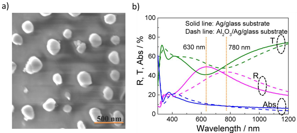
Fig.1 a) Surface morphology, b) reflectance (R), transmittance (T), absorption (Abs) of Ag nanoparticles on glass substrate
