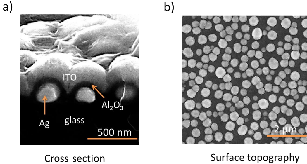
Fig.3 Morphologies of the structure of ITO/Al 2 O 3 /Ag/glass substrate
