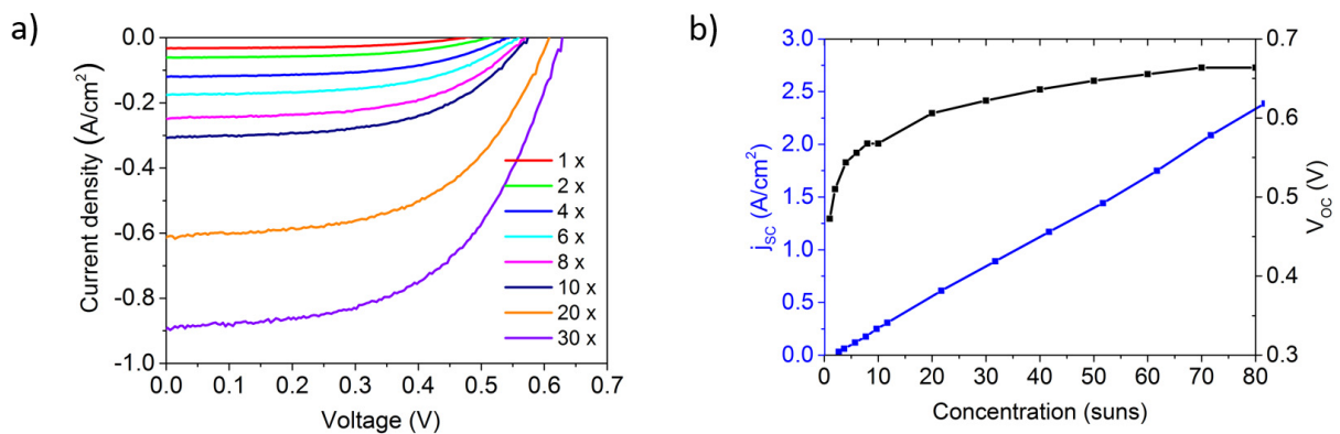
Figure 6. Electrical measurements of circular CIGSe micro solar cells sized 400\ \mu\text{m} in diameter and obtained in a top-down approach: a) jV characteristics for various concentration factors, b) j_{sc} and V_{oc} as a function of concentration.
