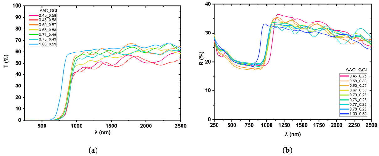
Figure S1. (a) Transmission curves of ACIGSe with high GGI (approx. 0.5 - 0.6) and varying AAC ratio; (b) Reflection curves of ACIGSe with low GGI (approx. 0.3) and varying AAC ratio.
